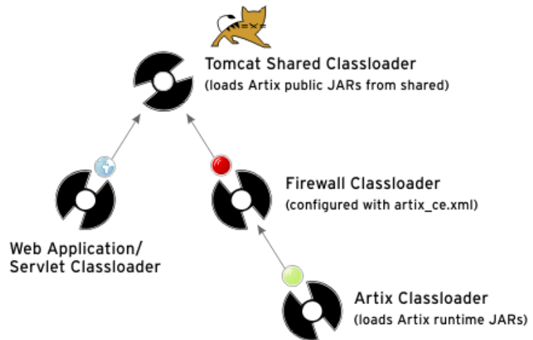
Figure 10: Classloader Configuration
